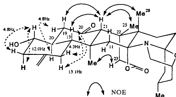
Fig. 4 : Stereochemistry of epinozoanthamine 7 .
